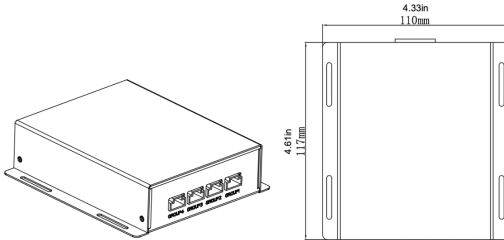
Driver Box & Dimensions
