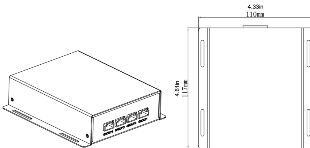
Driver Box & Dimensions
