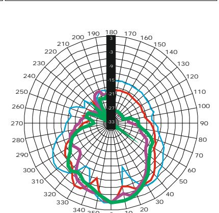
VERTICAL POLAR DIAGRAM — 1400 — 2000 — 2500 — 3150
